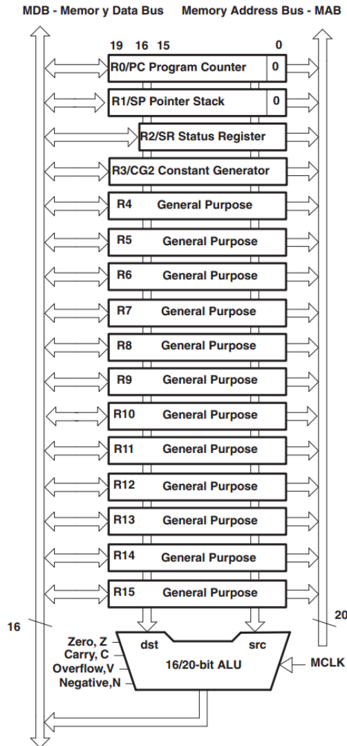
Figure 5.1: Memory address and data buses on the MSP430 source: [14]
