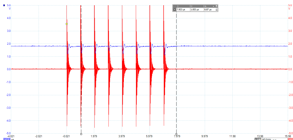
Figure 7.1: The glitch profile of the XMEGA64A3. The red line represents the digital glitch and the blue line represents the Vcc voltage.
