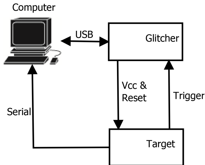
Figure 4.1: Schematic overview of the test setup
