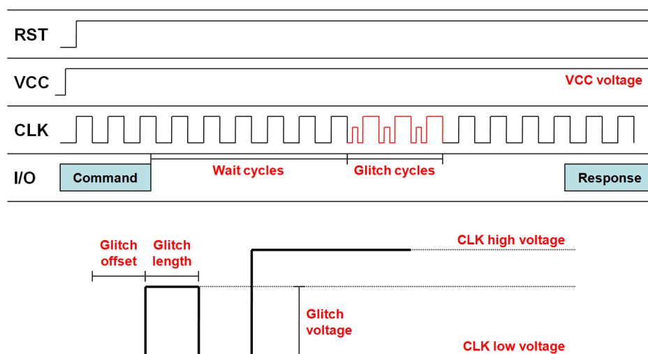
Figure 7.2: Glitch parameter timing
