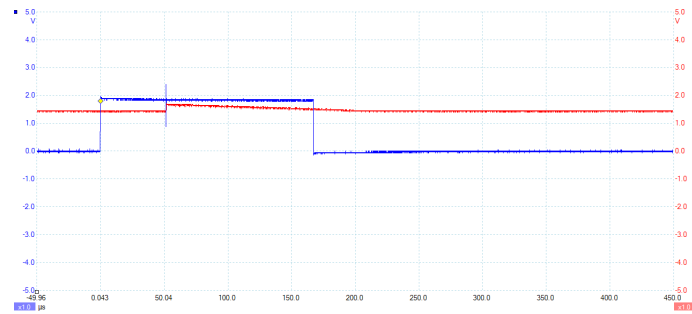
Figure 9.2: The red line represents the Vcore line and its reaction to a negative Vcc glitch
