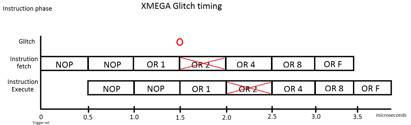
Figure 7.5: Timing model of a successful glitch
